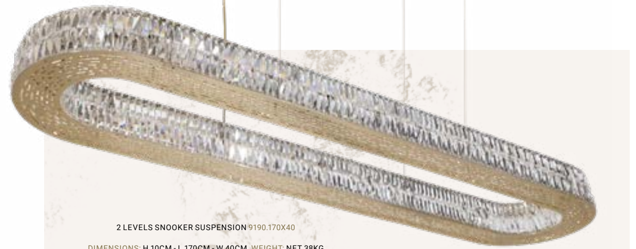
DIMENSIONS: H.10CM - L.170CM - W.40CM WEIGHT: NET 38KG BULBS: 22X G9 (28W) MATERIAL: BRASS & CRYSTAL
